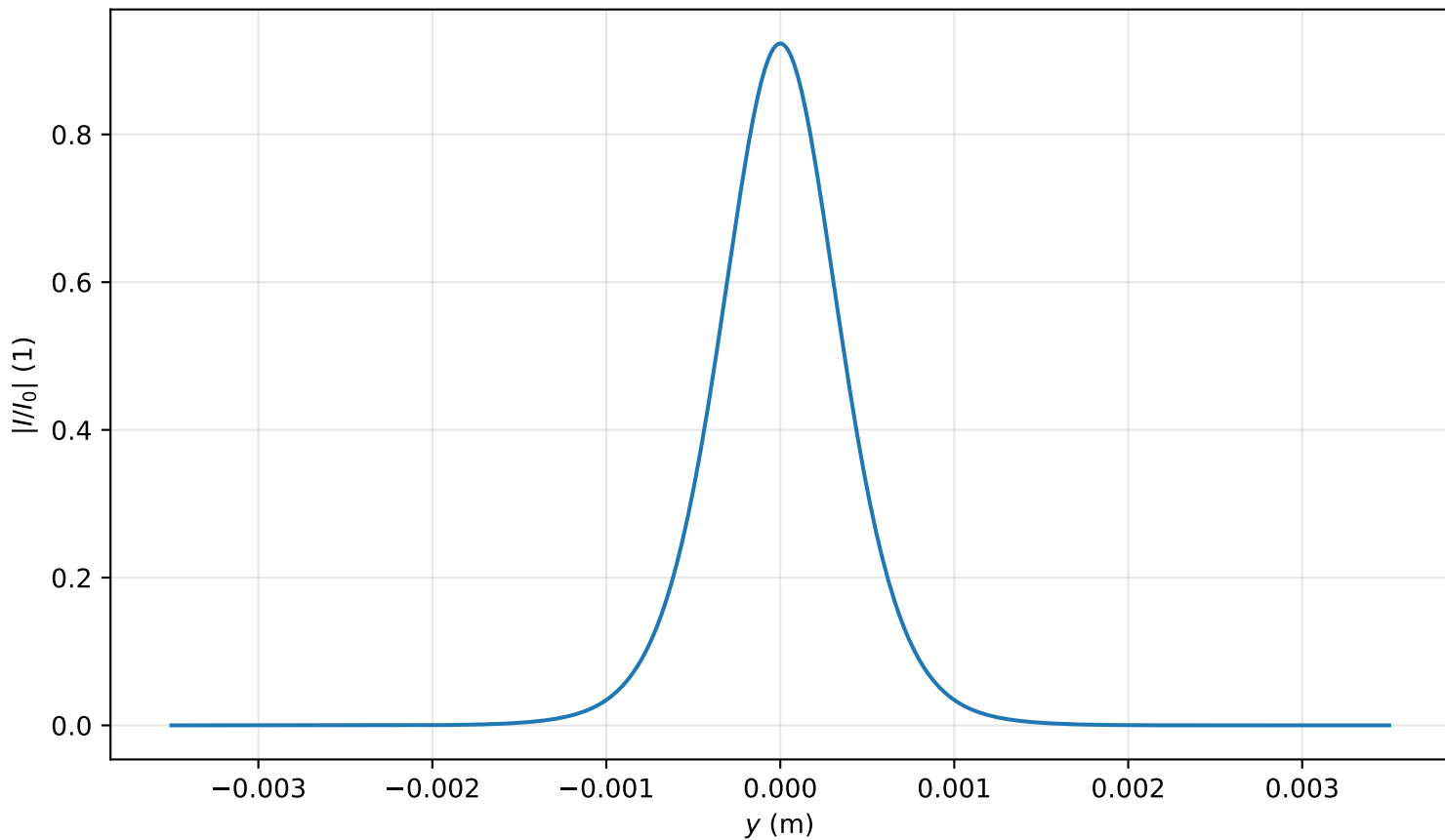
Intensity profile I(x = 0, y, z = 2.070)/I_0 , P_{in}=0.6P_{cr} , artificial time
